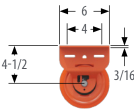
SLOTTED FOR 1/2" Ø BOLT
