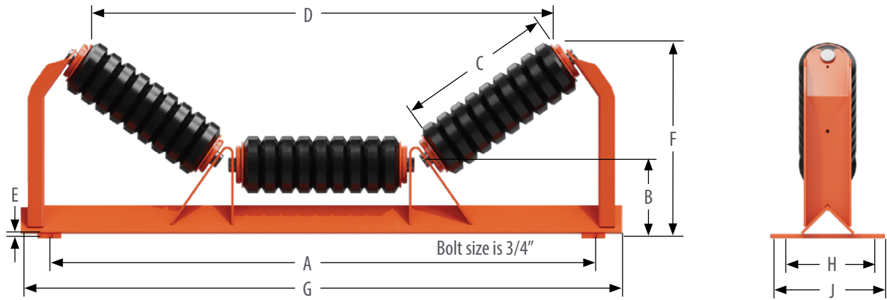
RUBBER CUSHION IMPACT TROUGHING IDLERS: 7" AND 8" DIAMETER
