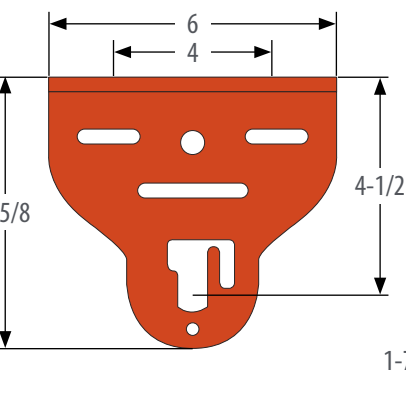
32-000017 4-1/2" Drop Bracket (1.63 lbs)*
