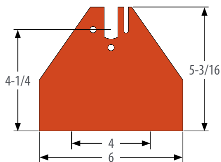
32-000019 4-1/4" Rise Bracket (2.94 lbs)*
