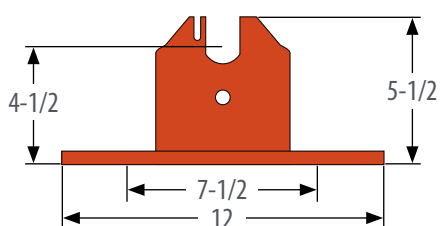
32-010040 1-1/2" Rise Bracket (5.31 lbs)
