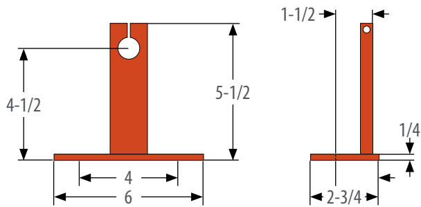
32-410450 4-1/2" CB Bracket (2.10 lbs)
