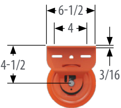
SLOTTED FOR 1/2" Ø BOLT
