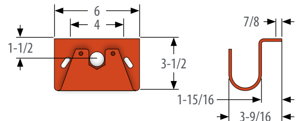
32-015120 1-1/2" Drop Hex Bracket (2.21 lbs)
