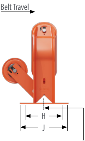
Center slot for single bolt mounting through 48" belt width
