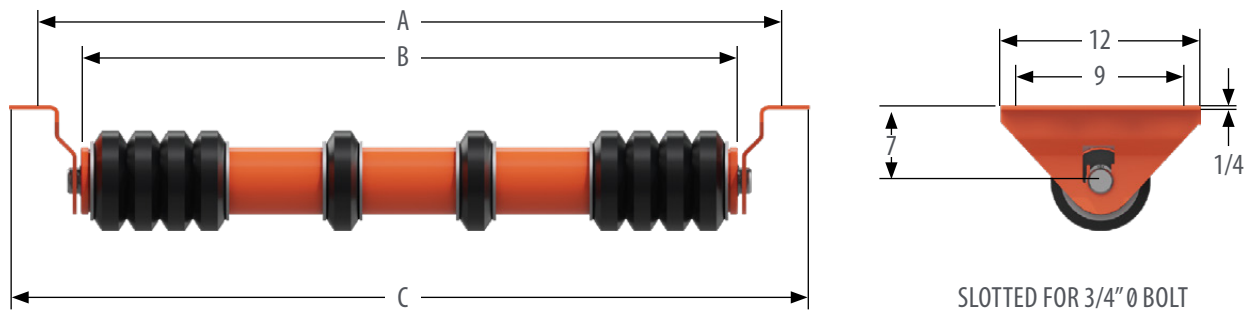
RUBBER CUSHION RETURN IDLERS: 6" AND 7" DIAMETER
