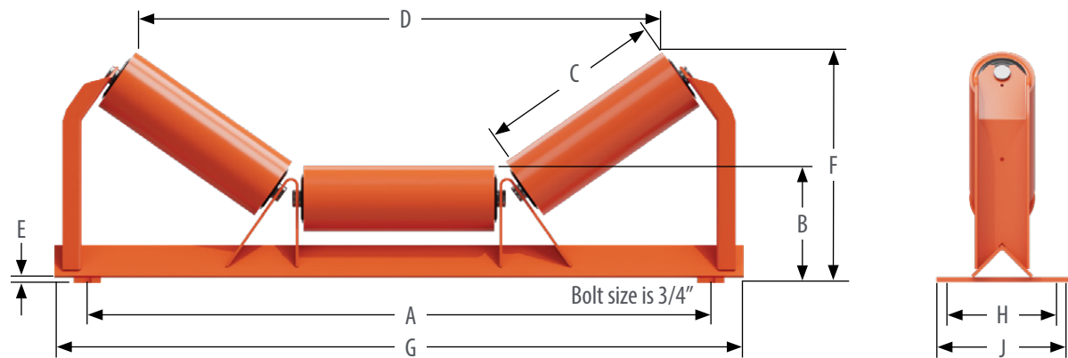
TRoughing IDLER (EQUAL LENGTH ROLLERS): 6" AND 7" DIAMETER
