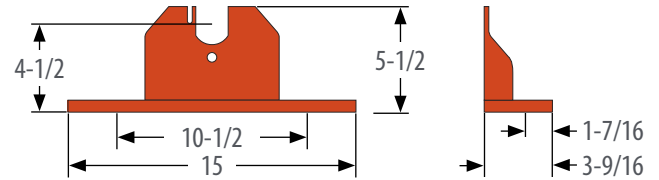
32-060002 CEMA F 4-1/2" Rise Bracket (10.00 lbs)
