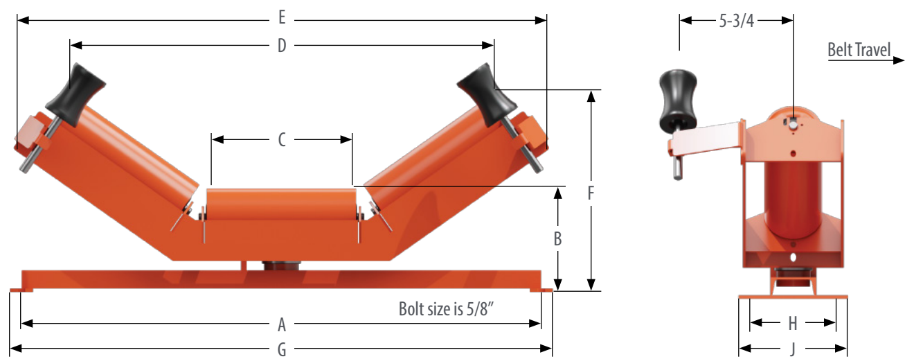
SELF-ALIGNING TROUGHING IDLERS: 5" AND 6" DIAMETER
