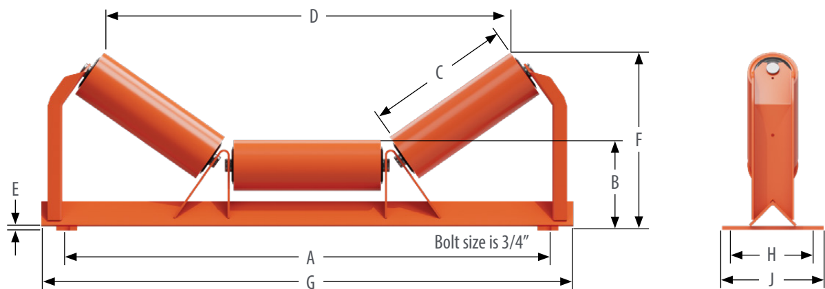
TROUGHING IDLER (EQUAL LENGTH ROLLERS): 6" AND 7" DIAMETER
