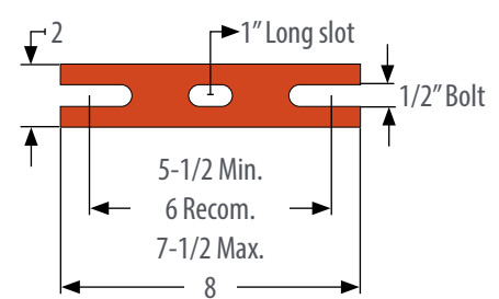
14"-36" BW CEMA B (0.97 lbs) 14"-20" BW CEMA C 33-018780
