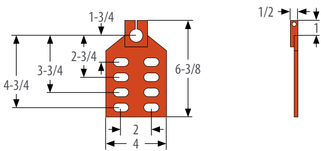
32-506000 CB Channel Mount Hex Bracket (2.00 lbs)
