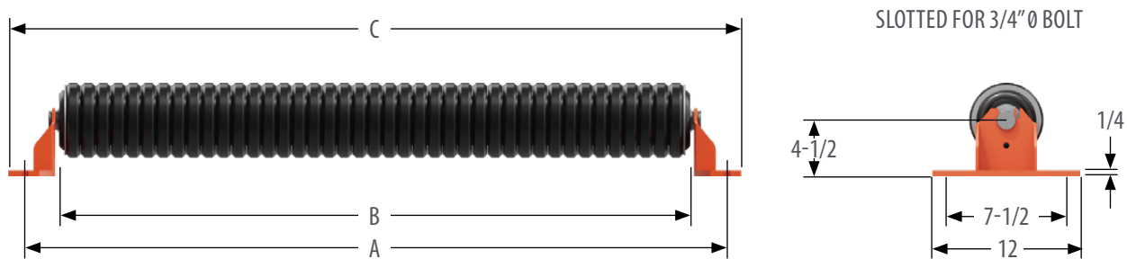
RUBBER CUSHION FLAT IDLERS: 6" AND 7" DIAMETER
