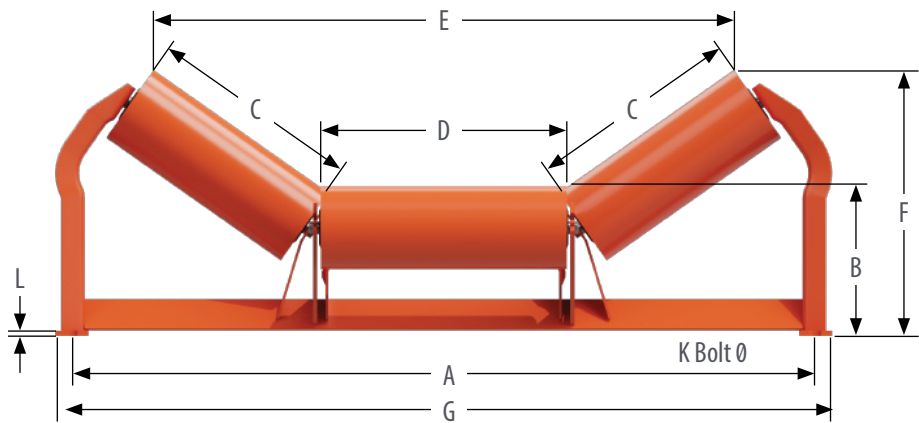
Center slot for single bolt mounting through 48" belt width
