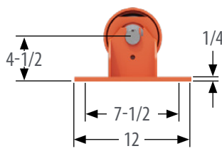
SLOTTED FOR 3/4" Ø BOLT
