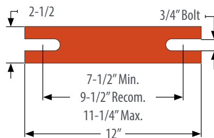
E, 40 DT, 45 DT 36"-72" BW 33-001001
